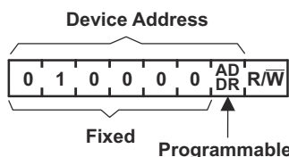
Figure 7-7. TCAL6408 Address
