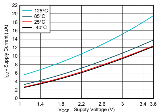
Figure 5-4. Supply Current vs Supply Voltage - FM mode
