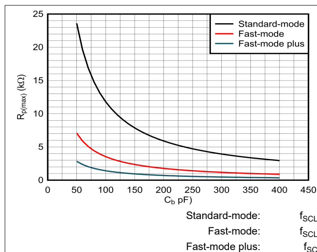
Figure 8-4. Maximum Pullup Resistance ( R_{p(max)} ) vs Bus Capacitance ( C_b )
