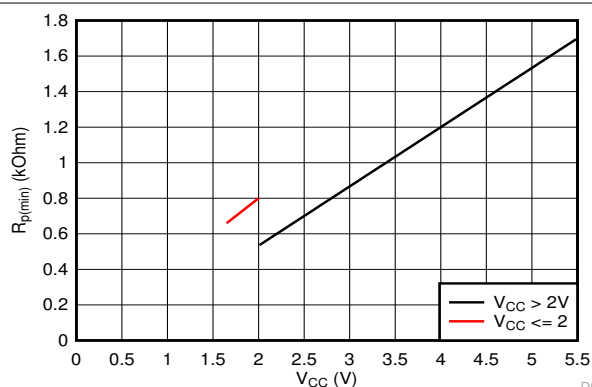
Figure 8-5. Minimum Pullup Resistance ( R_{p(min)} ) vs Pullup Reference Voltage ( V_{CC} )
