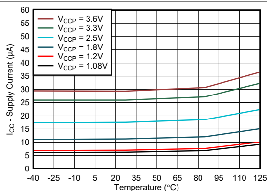
Figure 5-2. Supply Current vs Temperature - FM+ mode
