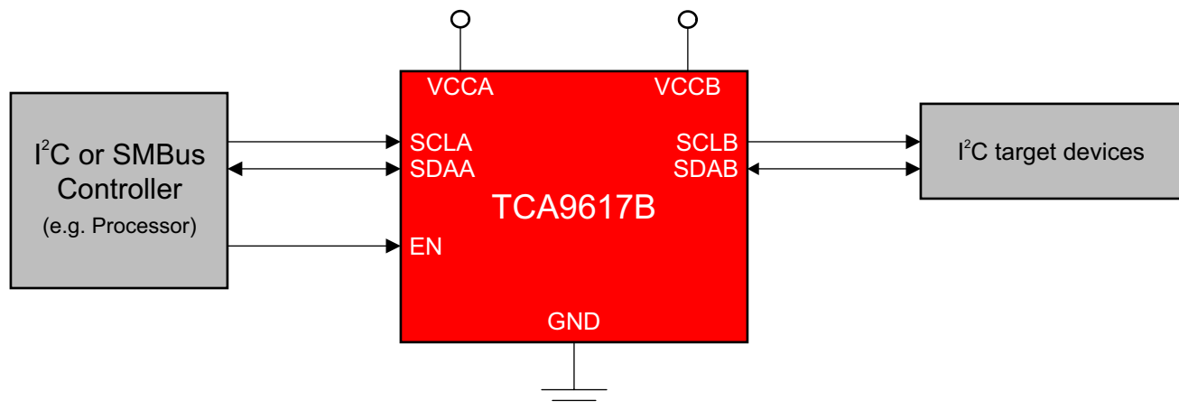
Simplified Schematic
