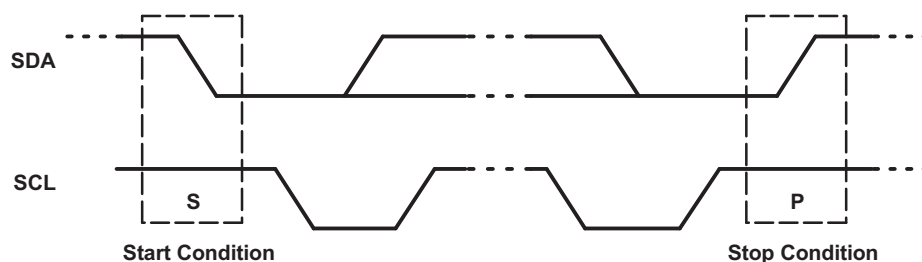
Figure 16. Definition of Start and Stop Conditions
