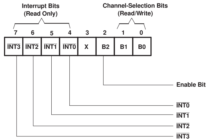
Figure 14. Control Register
