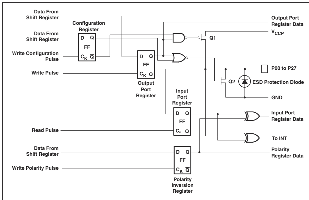
Figure 8-1. Positive Logic
