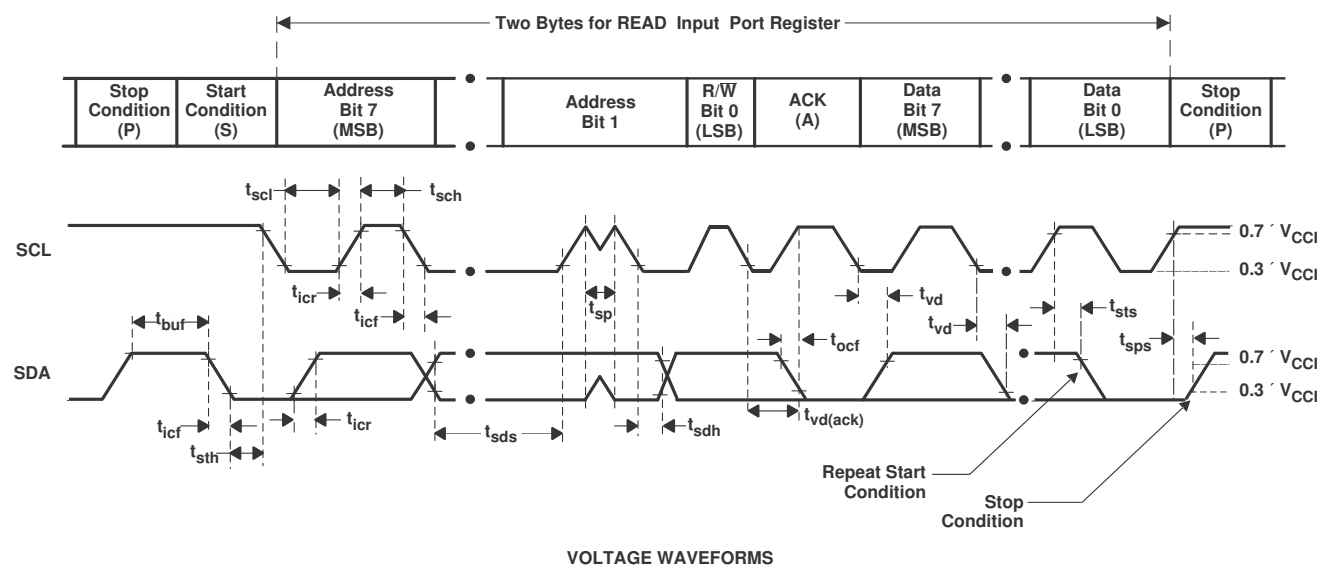
VOLTAGE WAVEFORMS
