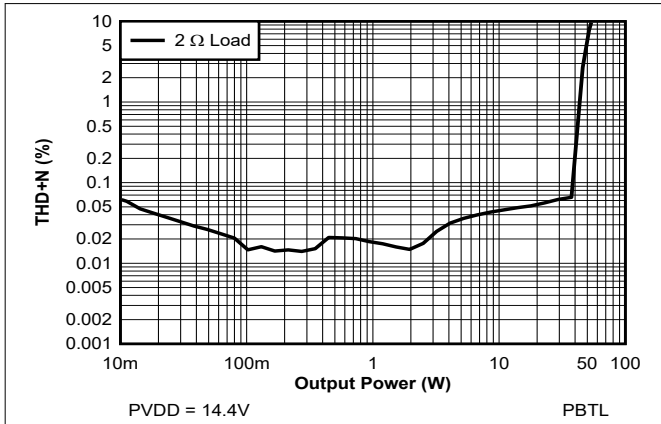
Figure 7-28. THD+N vs Power - PBTL - 14.4V
