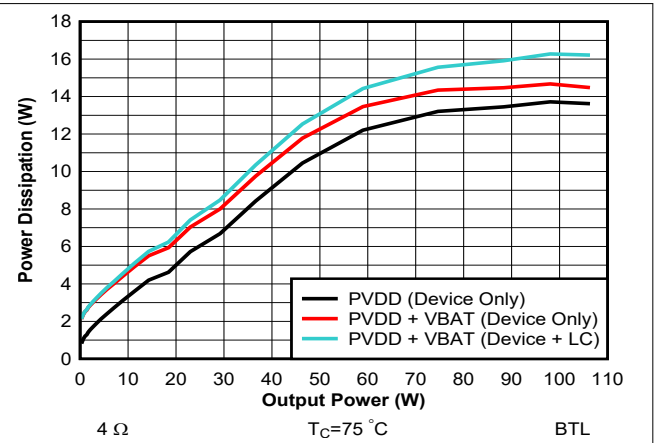
Figure 7-8. Power Dissipation vs Output Power - 14.4 V - 4 \Omega
