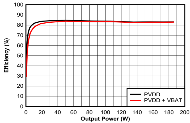
Figure 7-25. Efficiency vs Output Power - 2 \Omega - 384 kHz
