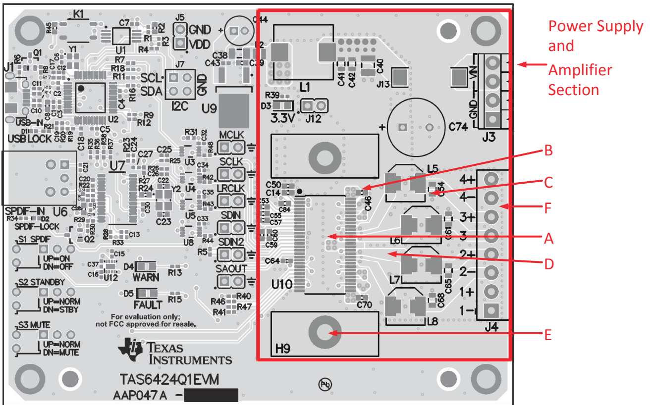
Figure 10-4. EVM Layout
