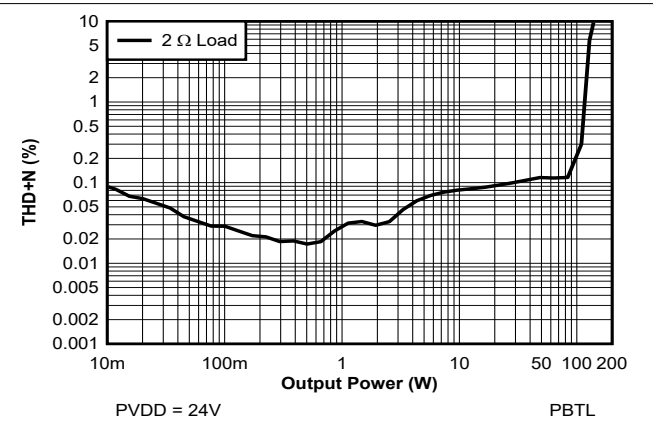
Figure 7-29. THD+N vs Power - PBTL - 24 V
