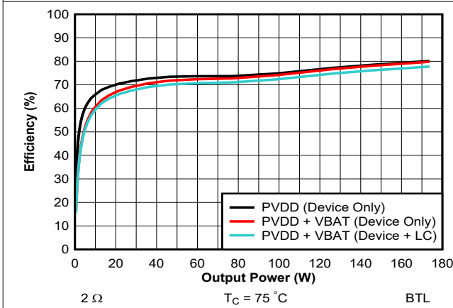
Figure 7-9. Efficiency vs Output Power - 14.4 V - 2 \Omega
