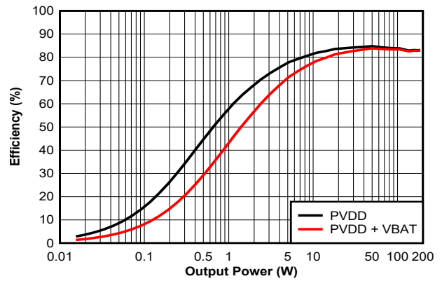
Figure 7-26. Efficiency vs Output Power - 2 \Omega - 384 kHz (Zoomed)
