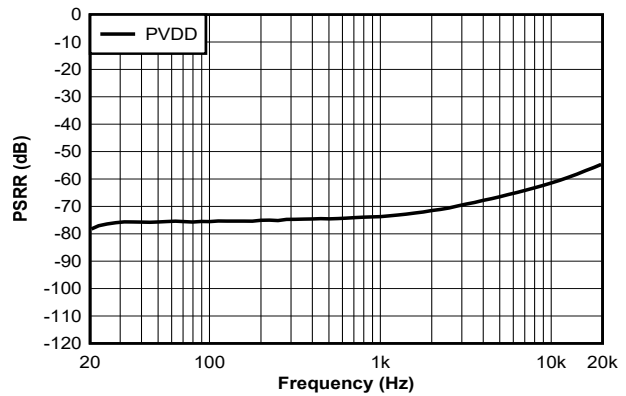
Figure 7-16. PSRR vs Frequency - PVDD Only
