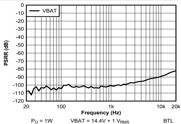
Figure 7-17. PSRR vs Frequency - VBAT Only
