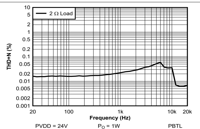
Figure 7-31. THD+N vs Frequency - PBTL - 24 V
