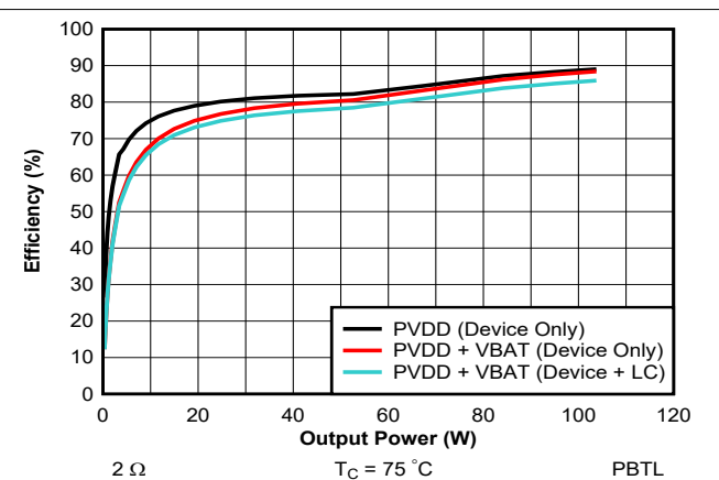
Figure 7-33. Efficiency vs Output Power - PBTL - 2 \Omega
