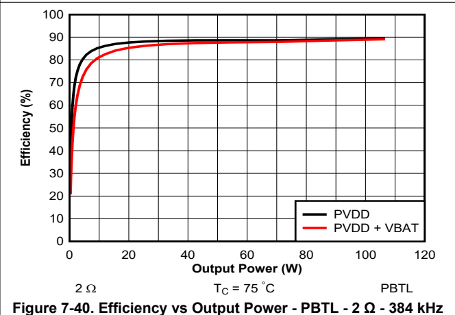
Figure 7-40. Efficiency vs Output Power - PBTL - 2 \Omega - 384 kHz
