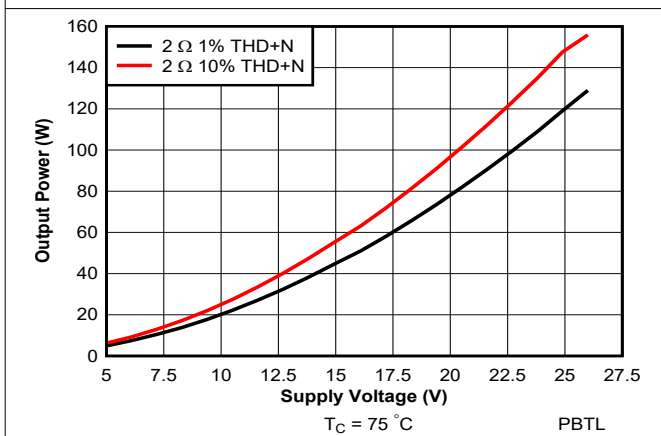
Figure 7-32. Output Power vs Supply Voltage - PBTL
