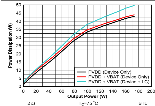
Figure 7-11. Power Dissipation vs Output Power - 14.4 V - 2 \Omega
