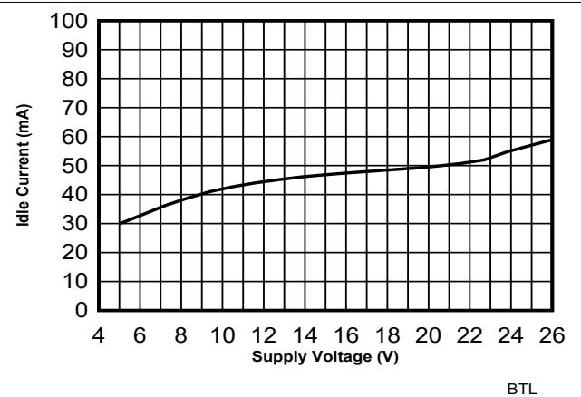
Figure 7-12. PVDD Idle Current vs Supply Voltage
