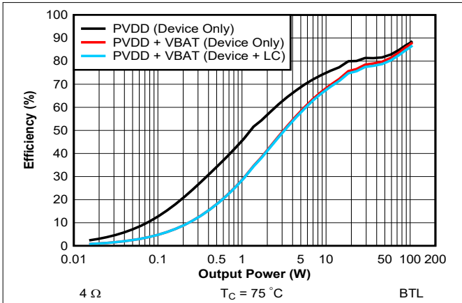
Figure 7-7. Efficiency vs Output Power - 14.4 V - 4 \Omega (Zoomed)
