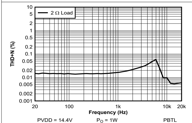
Figure 7-30. THD+N vs Frequency - PBTL - 14.4 V
