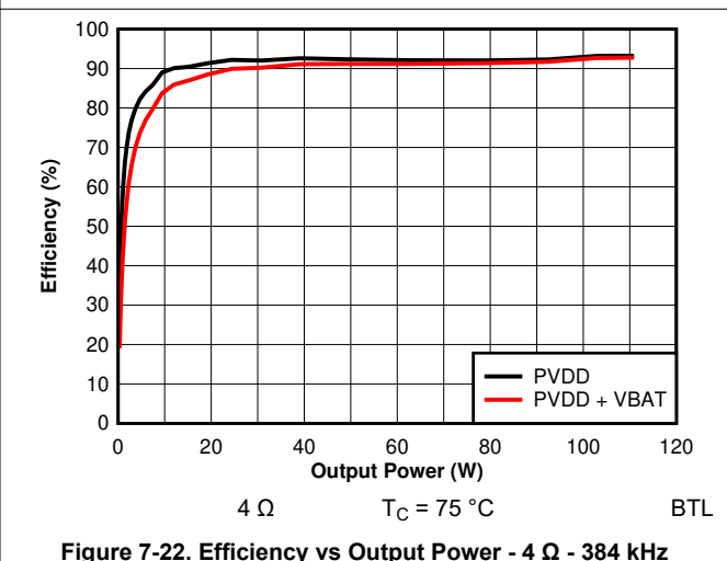
Figure 7-22. Efficiency vs Output Power - 4 \Omega - 384 kHz
