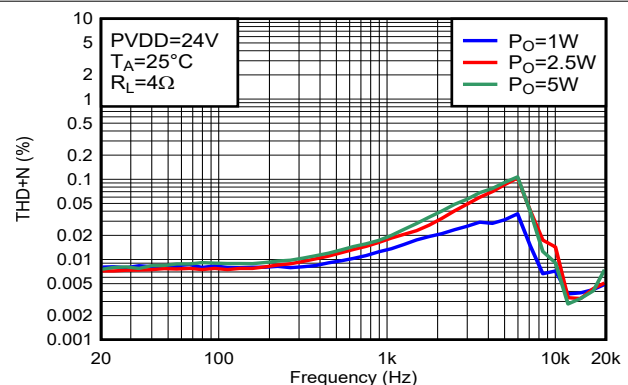
Figure 5-44. THD+N vs Frequency-PBTL
