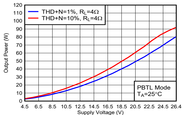
Figure 5-50. Output Power vs Supply Voltage
