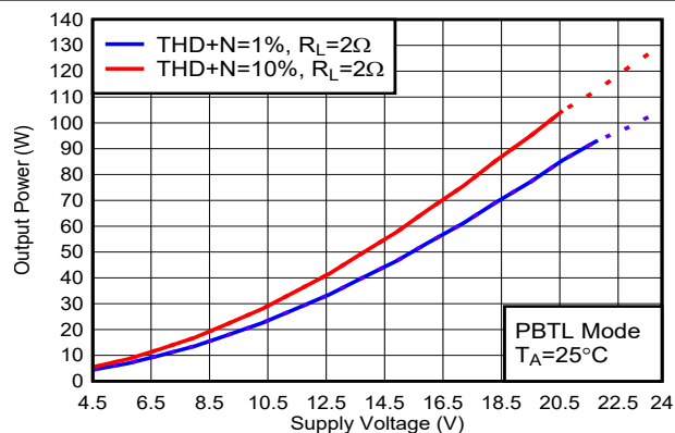
Figure 5-48. Output Power vs Supply Voltage
