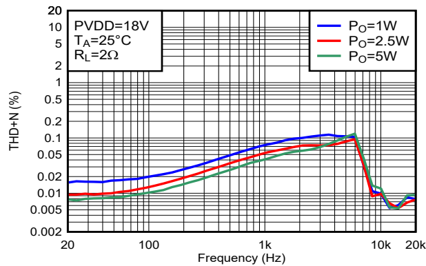
Figure 5-58. THD+N vs Frequency-PBTL
