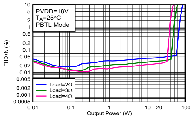
Figure 5-46. THD+N vs Output Power-PBTL
