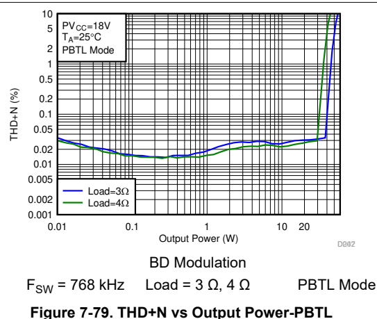
Figure 7-79. THD+N vs Output Power-PBTL
