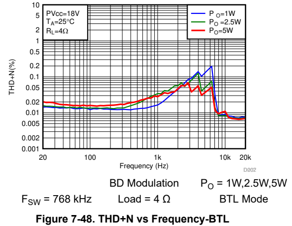
Figure 7-48. THD+N vs Frequency-BTL
