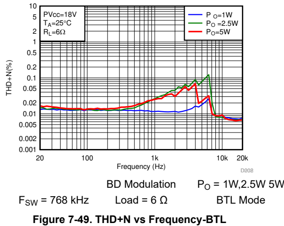
Figure 7-49. THD+N vs Frequency-BTL
