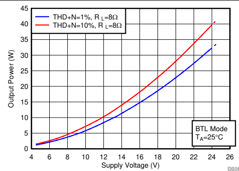
Figure 7-60. Output Power vs Supply Voltage
