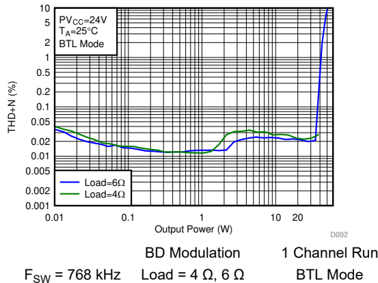
Figure 7-59. THD+N vs Output Power-BTL
