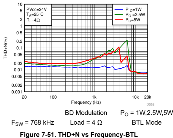
Figure 7-51. THD+N vs Frequency-BTL
