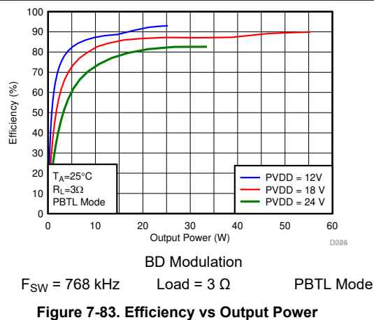
Figure 7-83. Efficiency vs Output Power
