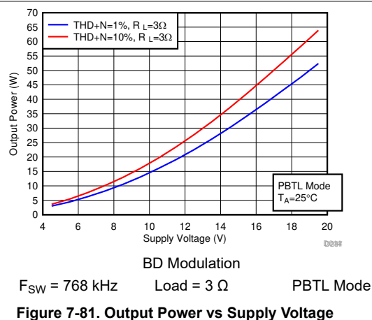
Figure 7-81. Output Power vs Supply Voltage
