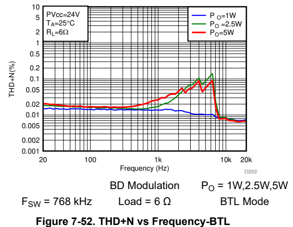
Figure 7-52. THD+N vs Frequency-BTL
