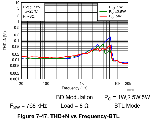
Figure 7-47. THD+N vs Frequency-BTL
