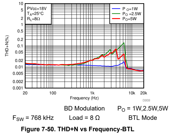
Figure 7-50. THD+N vs Frequency-BTL
