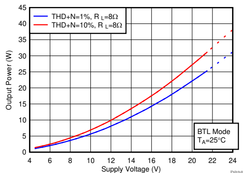
Figure 6-48. Output Power vs Supply Voltage
