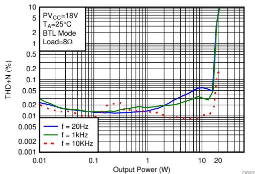
Figure 6-47. THD+N vs Output Power
