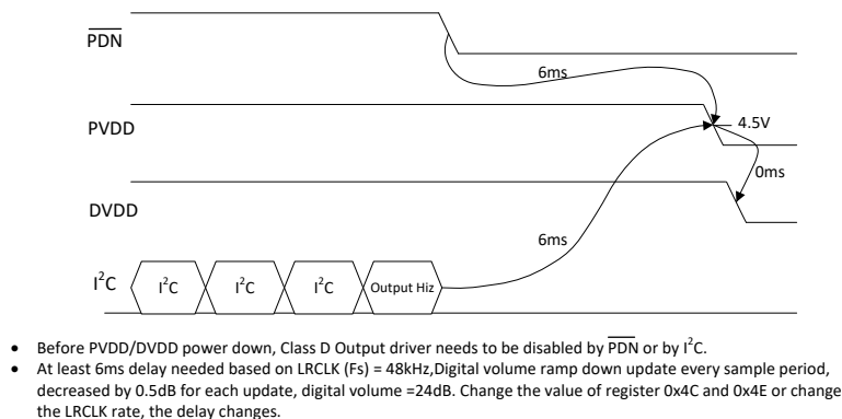
Figure 7-15. Power-Down Sequence
