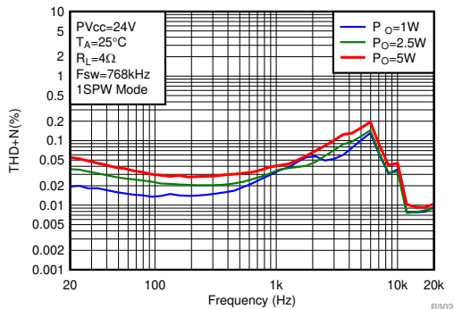
Figure 6-3. THD+N vs Frequency-BTL
