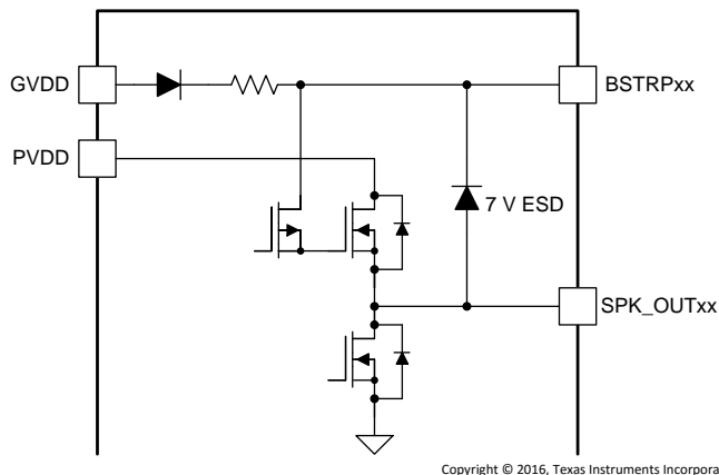
Figure 3. BSTRPx Pins
