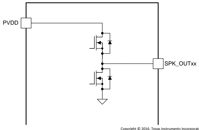
Figure 4. SPK_OUTxx Pins
