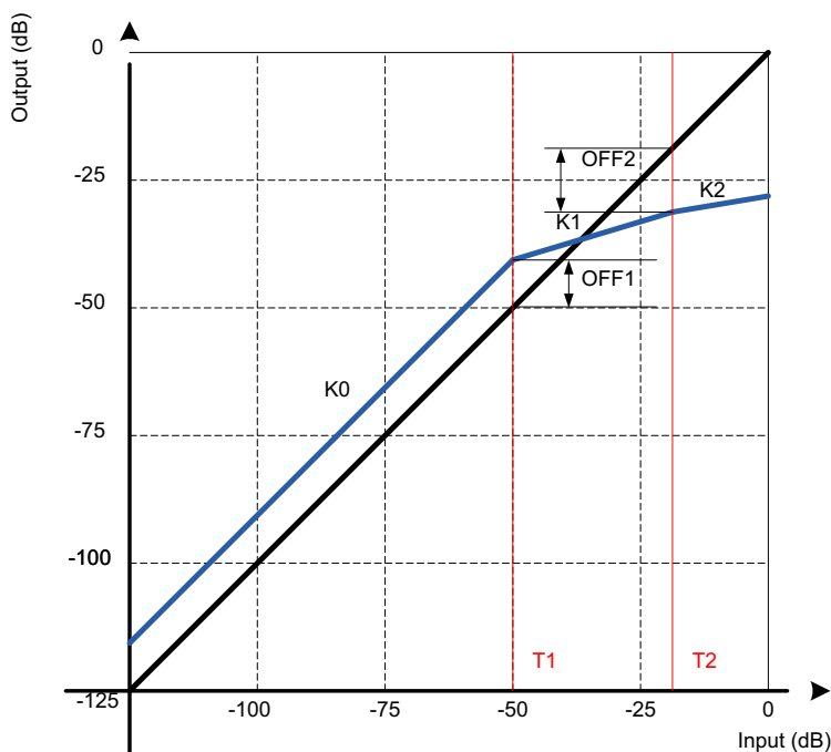
Figure 79. DRC Transfer Function Example Plot
