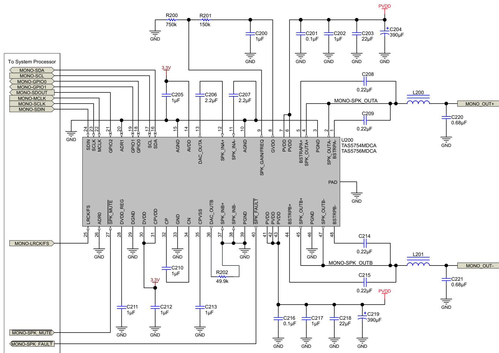
Figure 80. Mono (PBT) System Application Schematic
