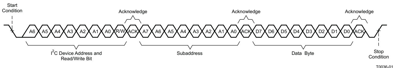
Figure 51. Single-Byte Write Transfer
