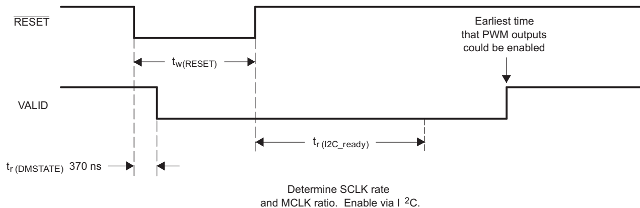
Figure 3. Reset Timing
