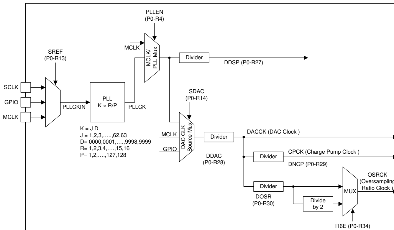
Figure 7-2. TAS3251 Clock Distribution Tree
