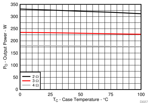
Figure 6-19. Output Power vs Temperature
