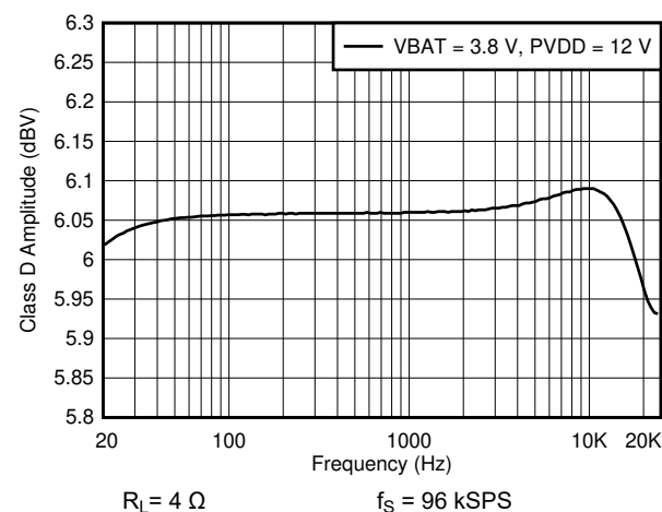
Figure 6-18. Class D Frequency Response
