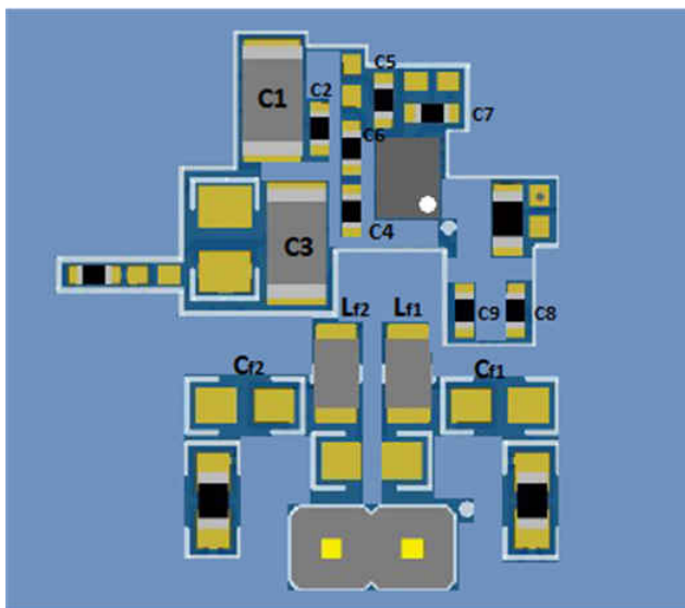
Figure 12-1. Component Placement
