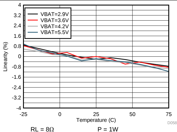
Figure 46. I-sense Linearity vs Temperature
