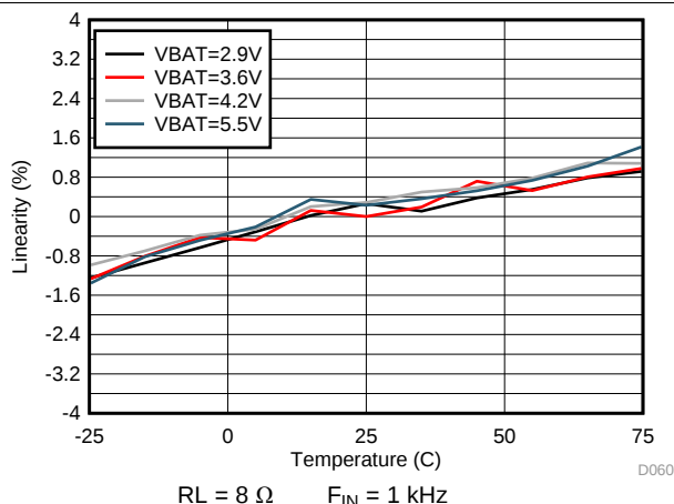
Figure 48. V/I-sense Linearity vs Temperature
