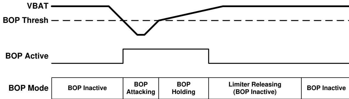
Figure 6-2. Brown Out Prevention Event
