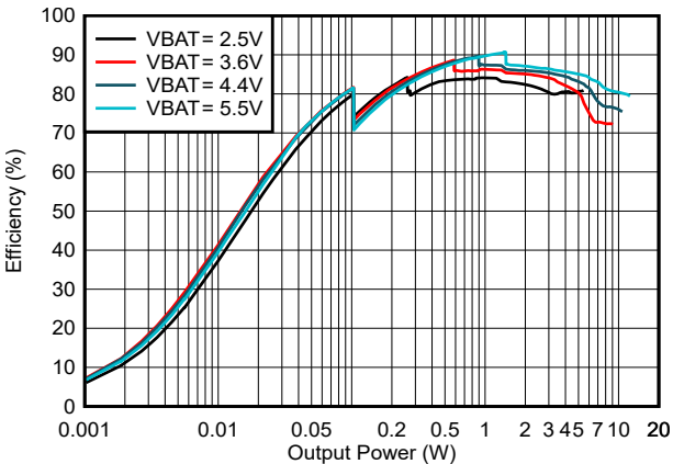
Figure 7-3. Efficiency vs Output Power
