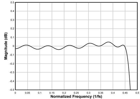
Figure 6-70. Linear-phase Decimation Filter Pass-Band Ripple
