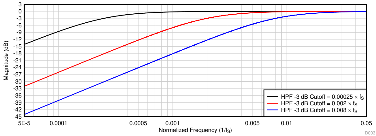
Figure 6-62. HPF Filter Frequency Response Plot
