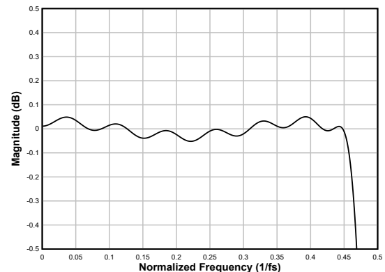
Figure 6-72. Linear-phase Decimation Filter Pass-Band Ripple
