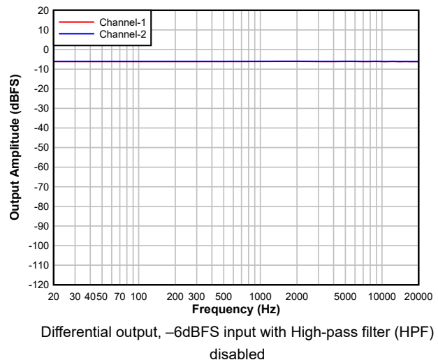
Figure 5-34. DAC Frequency Response
