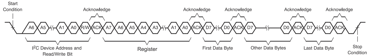
Figure 6-105. I 2 C Multiple-Byte Write Transfer
