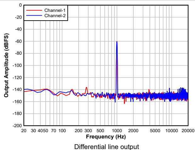
Figure 8-7. DAC FFT with -60dBFS Input
