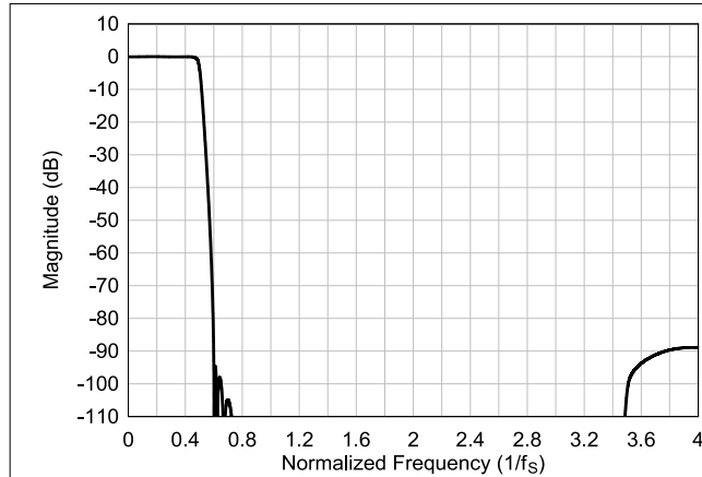
Figure 6-93. Ultra-Low-Latency interpolation Filter Magnitude Response
