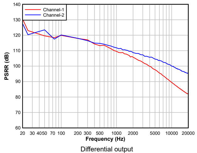
Figure 5-32. DAC PSRR vs Frequency
