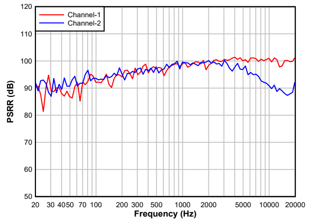
Figure 5-16. ADC PSRR vs Frequency
