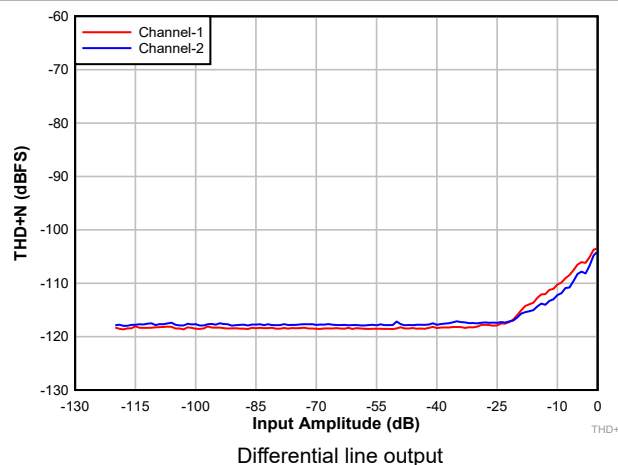
Figure 8-6. DAC THD+N Level vs Input
