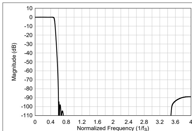
Figure 6-95. Ultra-Low-Latency interpolation Filter Magnitude Response
