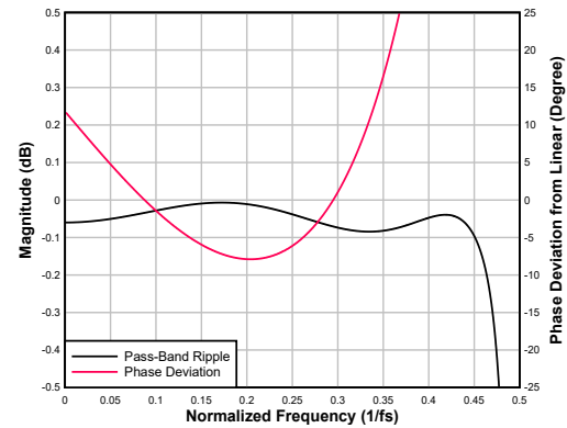
Figure 6-94. Ultra-Low-Latency interpolation Filter Pass-Band Ripple and Phase Deviation
