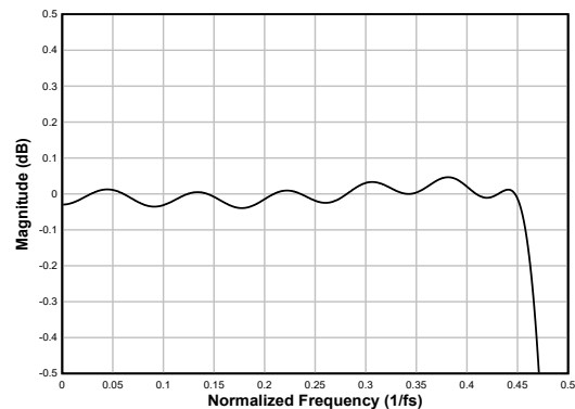
Figure 6-25. Linear Phase Decimation Filter Pass-Band Ripple
