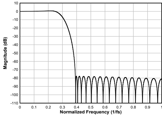
Figure 6-46. Linear Phase Interpolation Filter Magnitude Response
