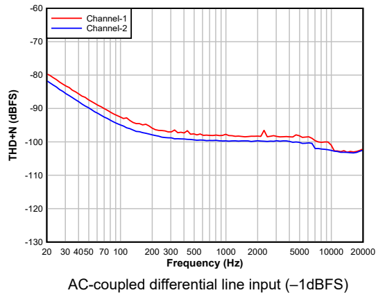
Figure 5-9. ADC THD+N vs Frequency
