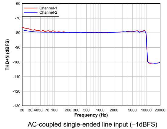
Figure 5-10. ADC THD+N vs Frequency
