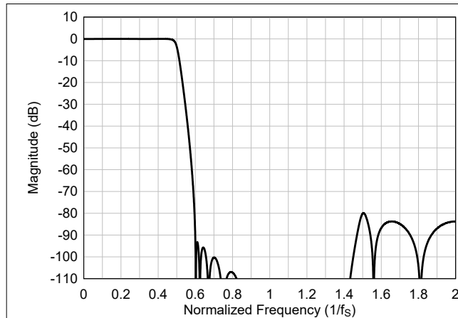
Figure 6-99. Ultra-Low-Latency interpolation Filter Magnitude Response
