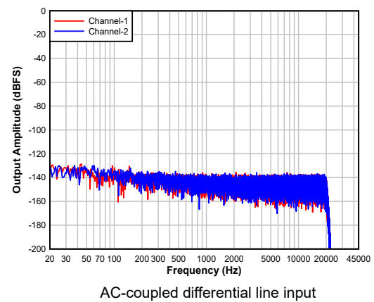
Figure 5-12. ADC FFT with Idle Channel Input
