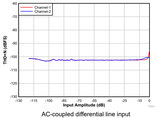
Figure 5-5. ADC THD+N Level vs Input
