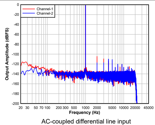
Figure 5-14. ADC FFT with -1dBFS Input
