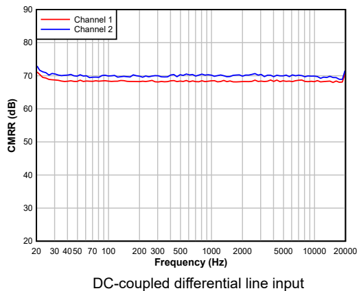
Figure 5-15. ADC CMRR vs Frequency
