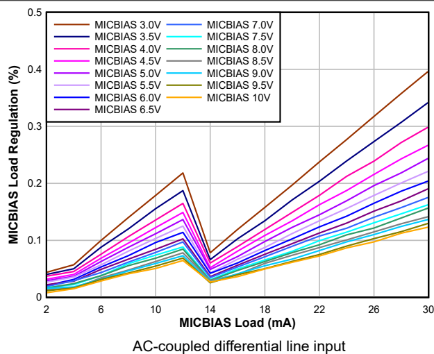
Figure 5-17. MICBIAS Load Regulation
