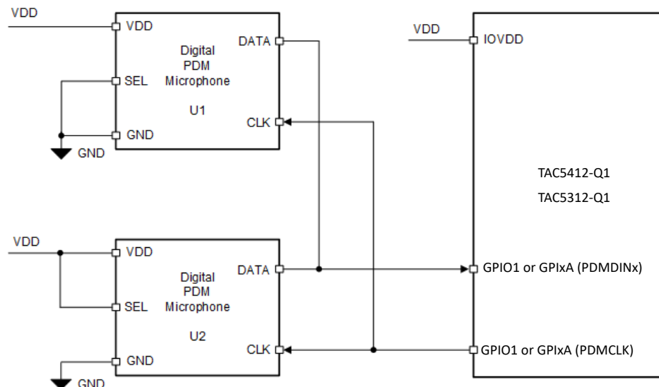
Figure 6-19. Digital PDM Microphones Connection Diagram for the TAC5312-Q1
