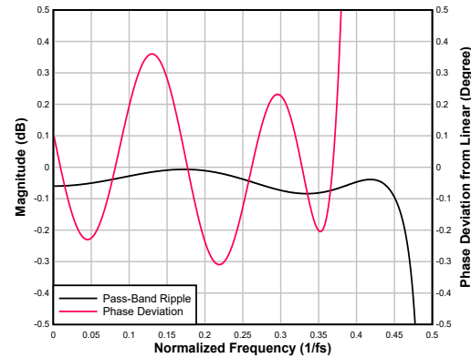
Figure 6-88. Low-latency Interpolation Filter Pass-Band Ripple and Phase Deviation
