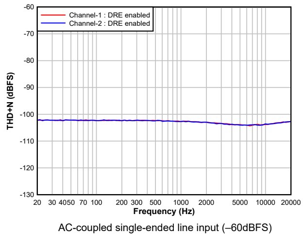
Figure 5-8. ADC A-weighted DR vs Frequency
