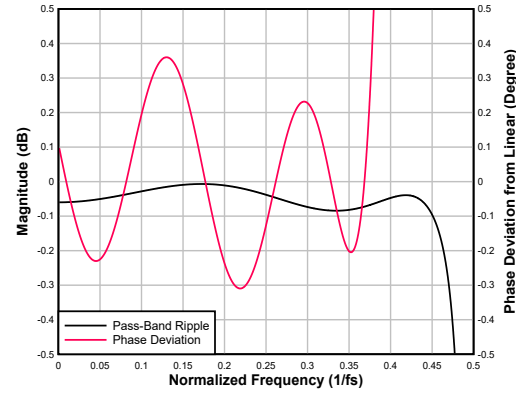
Figure 6-86. Low-latency Interpolation Filter Pass-Band Ripple and Phase Deviation
