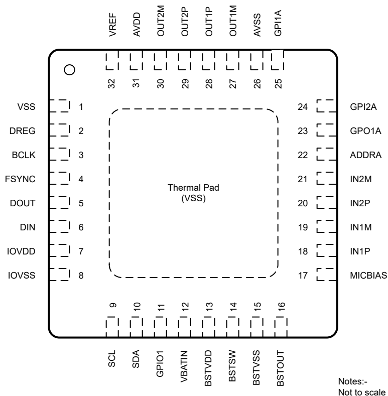
Figure 4-1. TAC5312-Q1 RTV Package, 32-Pin WQFN With Exposed Thermal Pad, Top View
