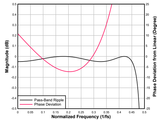
Figure 6-100. Ultra-Low-Latency interpolation Filter Pass-Band Ripple and Phase Deviation
