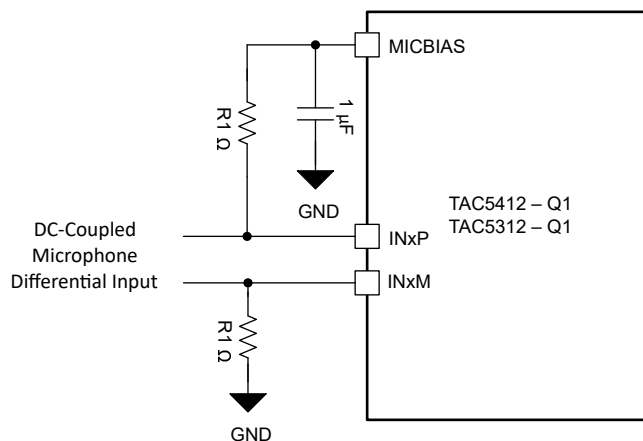
Figure 6-15. DC-Coupled Microphone or Line Differential Input Connection
