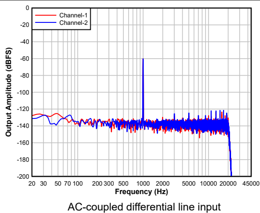
Figure 5-13. ADC FFT with -60dBFS Input
