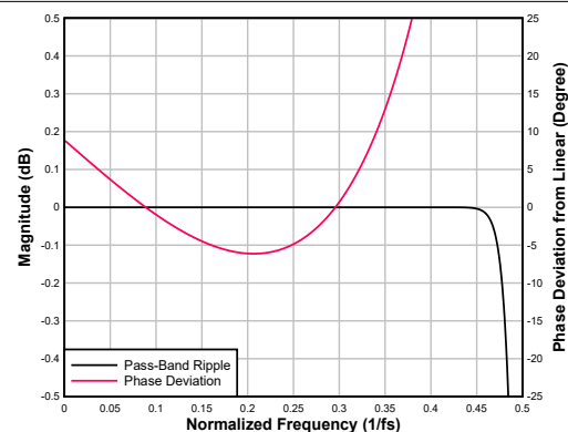
Figure 6-102. Ultra-Low-Latency interpolation Filter Pass-Band Ripple and Phase Deviation
