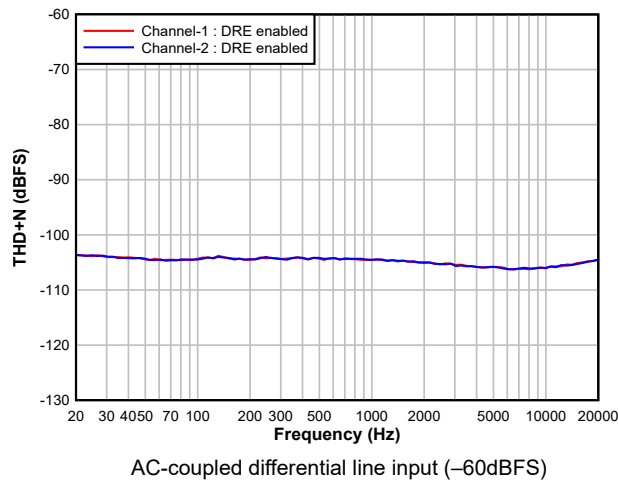
Figure 5-7. ADC A-weighted DR vs Frequency
