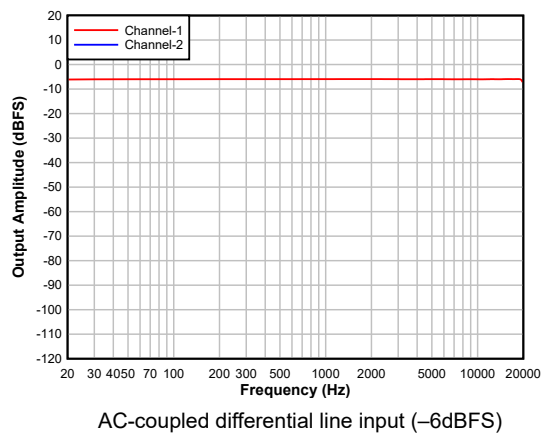
Figure 5-11. ADC Frequency Response
