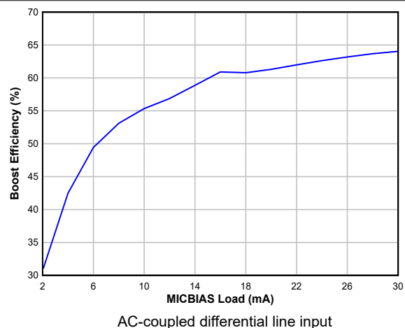
Figure 5-18. Boost Efficiency vs MICBIAS Load Current
