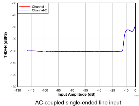
Figure 5-6. ADC THD+N Level vs Input
