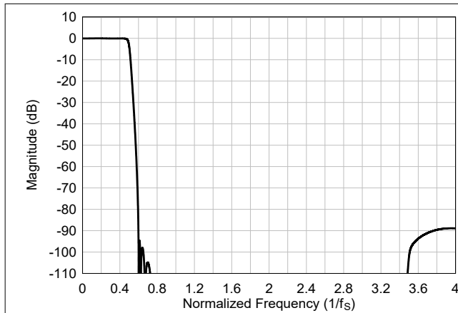
Figure 7-103. Ultra-Low-Latency interpolation Filter Magnitude Response
