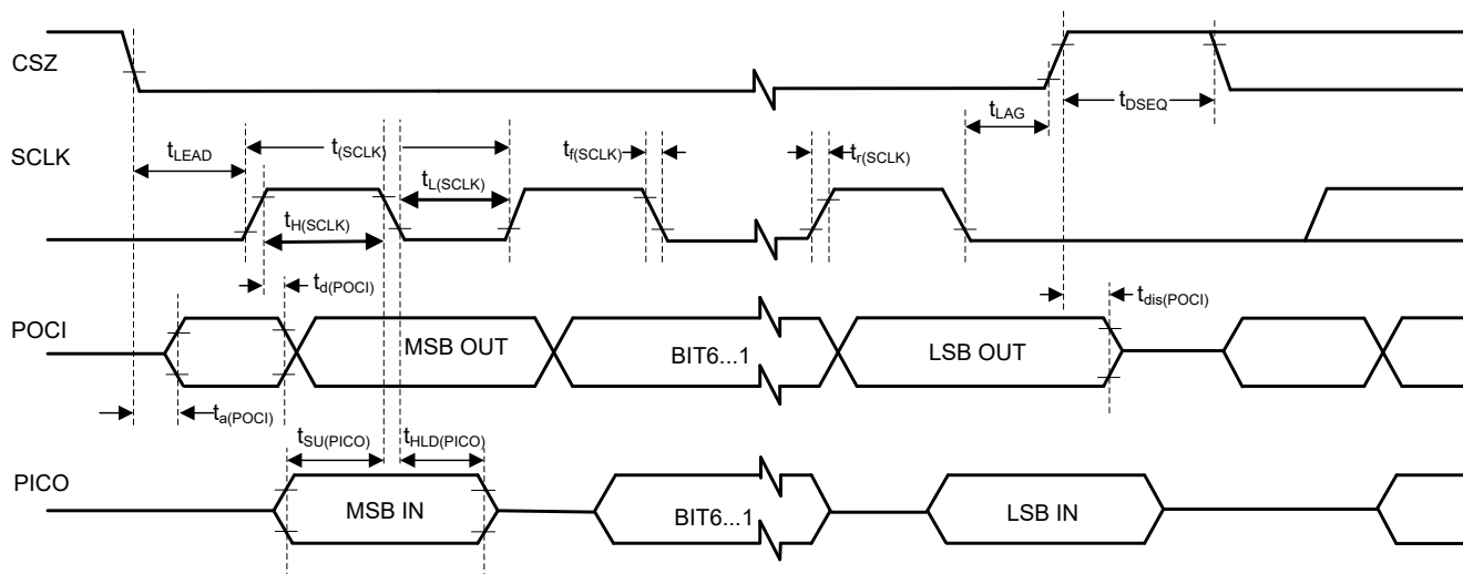
Figure 6-2. SPI Interface Timing Diagram
