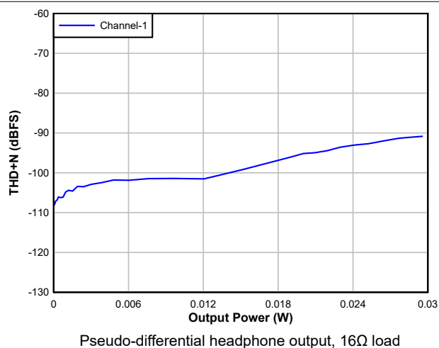
Figure 6-24. DAC THD+N Level vs output power
