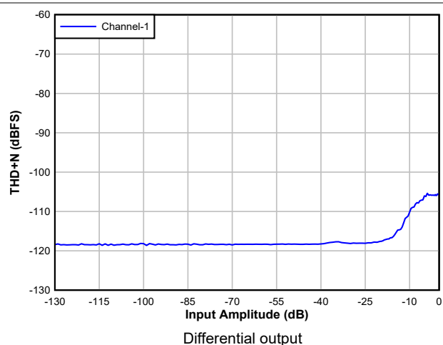
Figure 6-19. DAC THD+N Level vs Input
