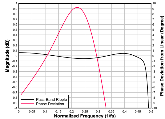
Figure 7-57. Low-latency Decimation Filter Pass-Band Ripple and Phase Deviation
