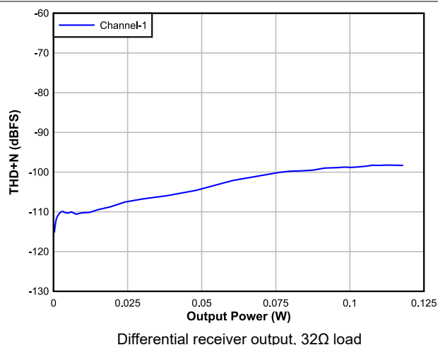
Figure 6-22. DAC THD+N Level vs output power
