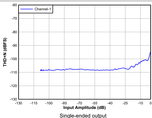
Figure 6-20. DAC THD+N Level vs Input
