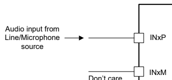
Figure 7-18. Single-ended DC-Coupled Input Connection (ADC_CHx_INSRC set to 2'b01 and ADC_CHx_CM_TOL set to 2'b01 or 2'10)
