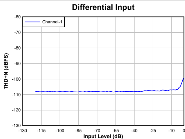
Figure 6-6. ADC THD+N Level vs Input
