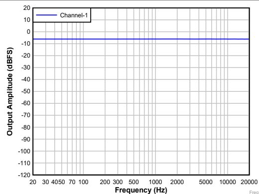
Figure 5-34. DAC Frequency Response
