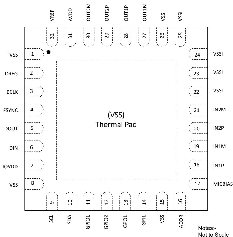
Figure 4-1. TAC5111-Q1 RTV Package, 32-Pin WQFN With Exposed Thermal Pad, Top View
