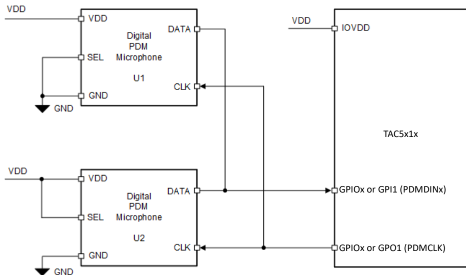
Figure 6-25. Digital PDM Microphones Connection Diagram for the TAC5111-Q1
