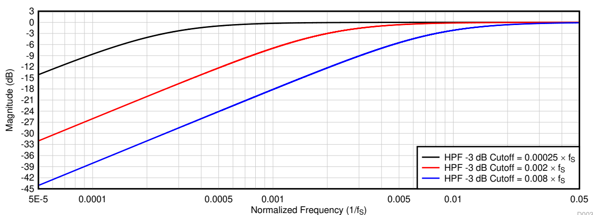
Figure 6-28. HPF Filter Frequency Response Plot
