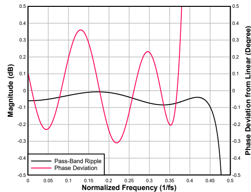
Figure 6-92. Low-latency Interpolation Filter Pass-Band Ripple and Phase Deviation
