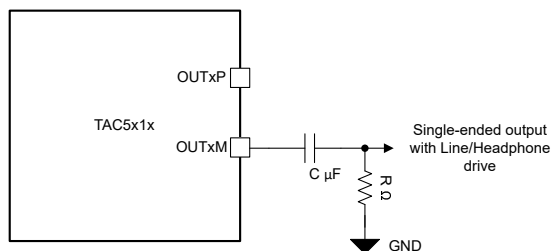
Figure 6-23. Mono Single-ended Output Connection on OUT1M (OUT1x_CFG[2:0] = 3'b011)
