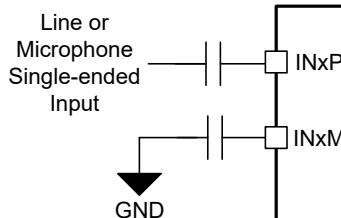
Figure 6-17. Single-ended AC-Coupled Input Connection (ADC_CHx_INSRC set to 2'b01 and ADC_CHx_CM_TOL set to 2'b00 or 2'b01 or 2'10)
