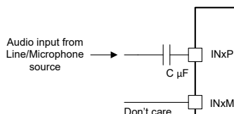
Figure 6-17. Single-ended AC-Coupled Input Connection (ADC_CHx_INSRC set to 2'b01 and ADC_CHx_CM_TOL set to 2'b00 or 2'b01 or 2'10)
