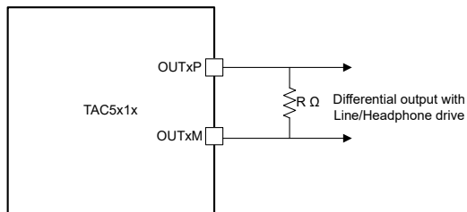
Figure 6-21. Differential Output Connection (OUT1x_CFG[2:0] = 3'b000)
