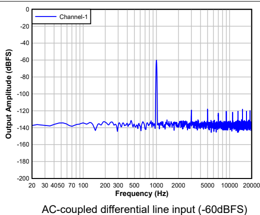
Figure 8-2. ADC FFT with -60dBFS Input
