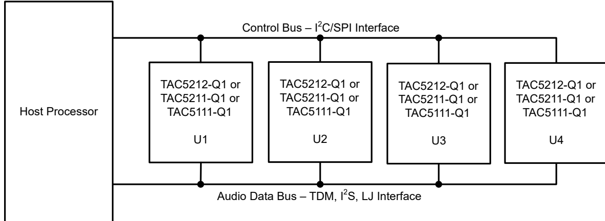
Figure 6-14. Multiple TAC5111-Q1 Devices With Shared Control and Audio Data Buses
