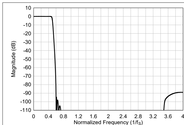
Figure 6-101. Ultra-Low-Latency interpolation Filter Magnitude Response
