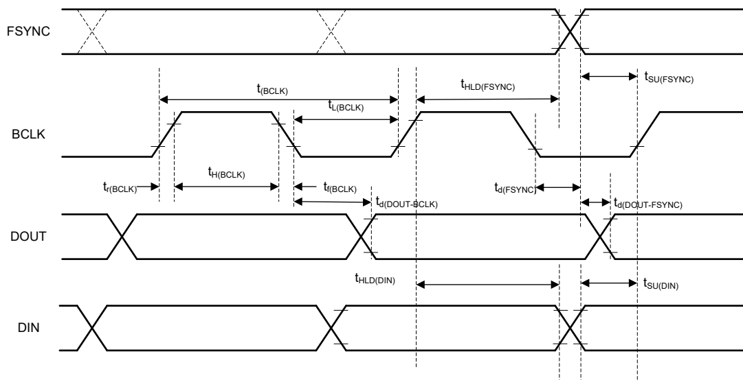
Figure 5-3. TDM (With BCLK_POL = 1), I 2 S, and LJ Interface Timing Diagram
