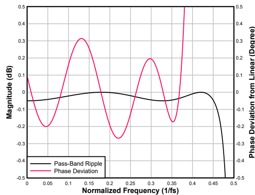
Figure 6-96. Low-latency Interpolation Filter Pass-Band Ripple and Phase Deviation
