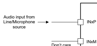
Figure 6-18. Single-ended DC-Coupled Input Connection (ADC_CHx_INSRC set to 2'b01 and ADC_CHx_CM_TOL set to 2'b01 or 2'10)
