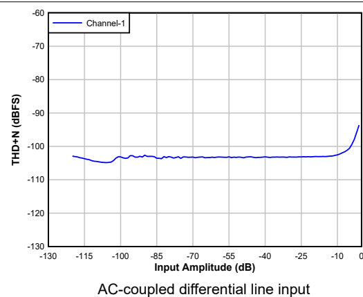
Figure 8-3. ADC THD+N Level vs Input
