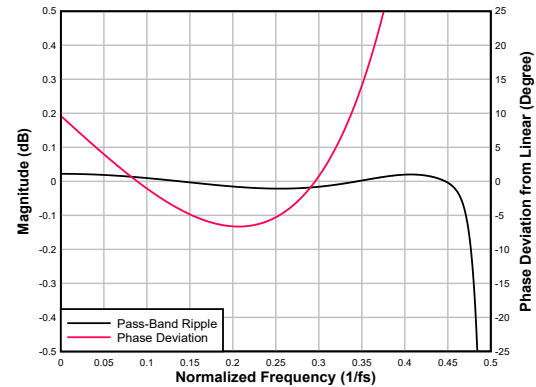
Figure 6-63. Ultra Low-latency Decimation Filter Pass-Band Ripple and Phase Deviation
