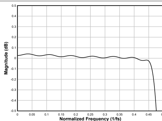
Figure 6-31. Linear-phase Decimation Filter Pass-Band Ripple
