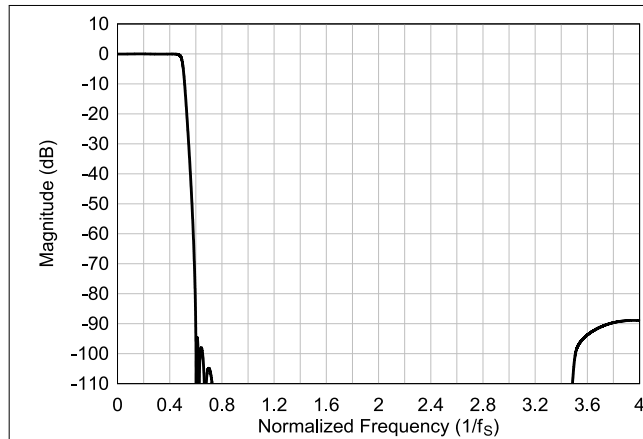
Figure 6-99. Ultra-Low-Latency interpolation Filter Magnitude Response
