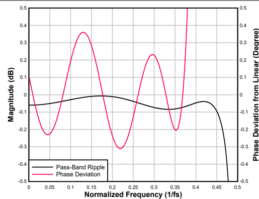
Figure 6-94. Low-latency Interpolation Filter Pass-Band Ripple and Phase Deviation
