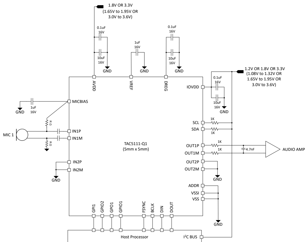
Figure 8-1. Mono Microphone with Mono Lineout Block Diagram
