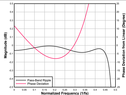
Figure 6-102. Ultra-Low-Latency interpolation Filter Pass-Band Ripple and Phase Deviation
