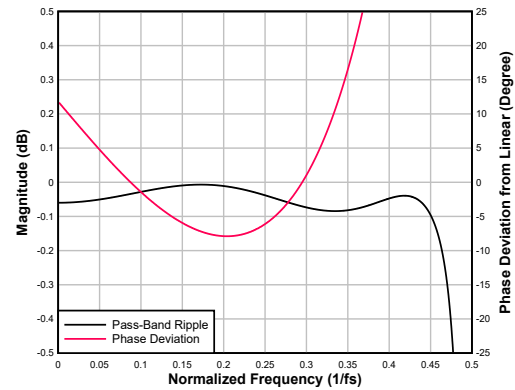
Figure 6-100. Ultra-Low-Latency interpolation Filter Pass-Band Ripple and Phase Deviation
