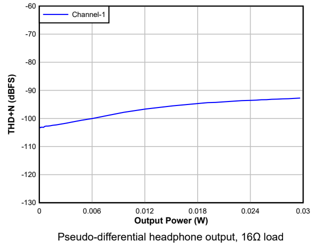
Figure 6-24. DAC THD+N Level vs output power
