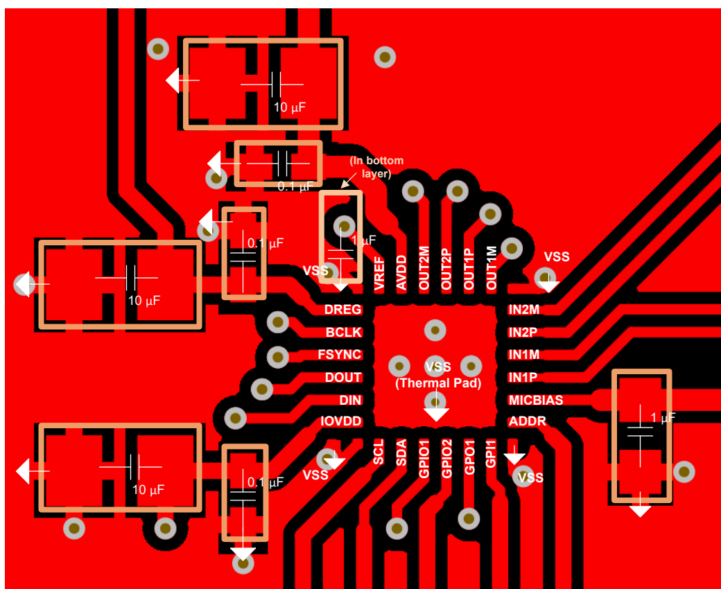
Figure 9-7. Example Layout
