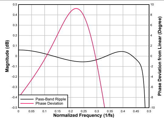
Figure 6-50. Low-latency Decimation Filter Pass-Band Ripple and Phase Deviation
