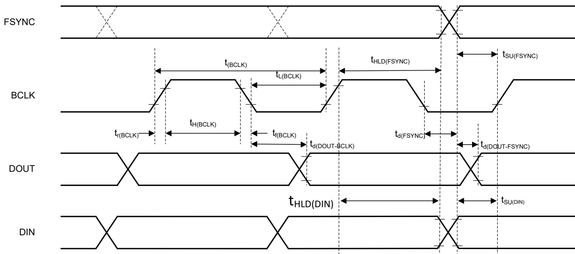
Figure 5-3. TDM, I²S, LJ Interface Timing Diagram
