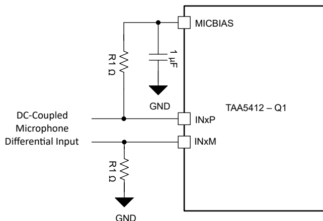
Figure 6-14. DC-Coupled Microphone Differential Input Connection
