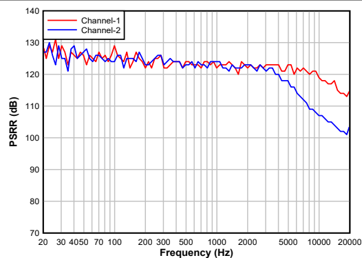
Figure 5-18. ADC PSRR vs Frequency
