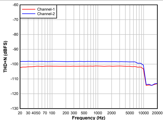
Figure 5-11. ADC THD+N vs Frequency
