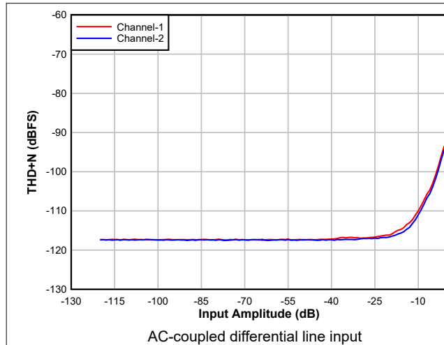
Figure 8-2. ADC THD+N Level vs Input
