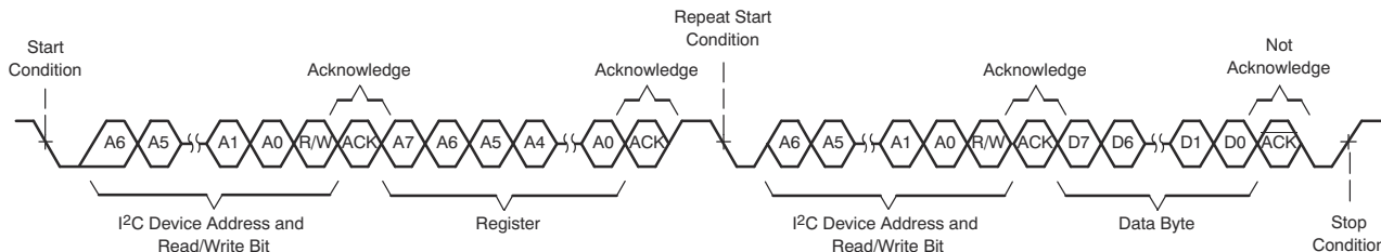
Figure 6-68. I 2 C Single-Byte Read Transfer
