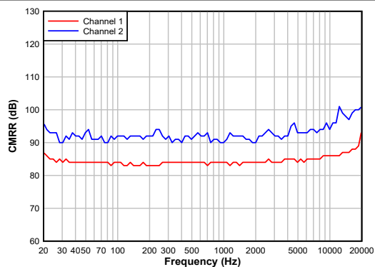
Figure 5-17. ADC CMRR vs Frequency
