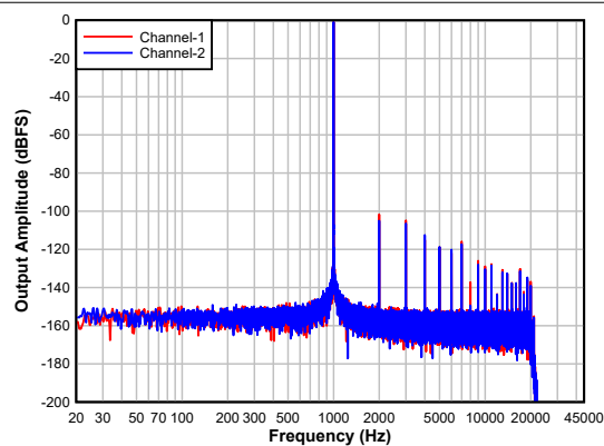
Figure 5-16. AD FFT with -1dBFS Input
