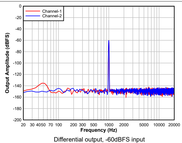
Figure 8-3. ADC FFT with -60dBFS Input
