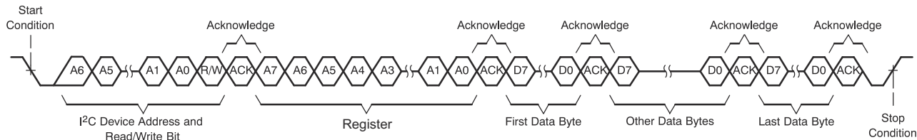
Figure 6-67. I 2 C Multiple-Byte Write Transfer
