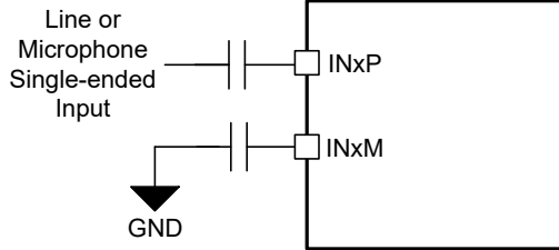
Figure 6-17. Single-ended AC-Coupled Input Connection (ADC_CHx_INSRC set to 2'b01 and ADC_CHx_CM_TOL set to 2'b00 or 2'b01 or 2'10)
