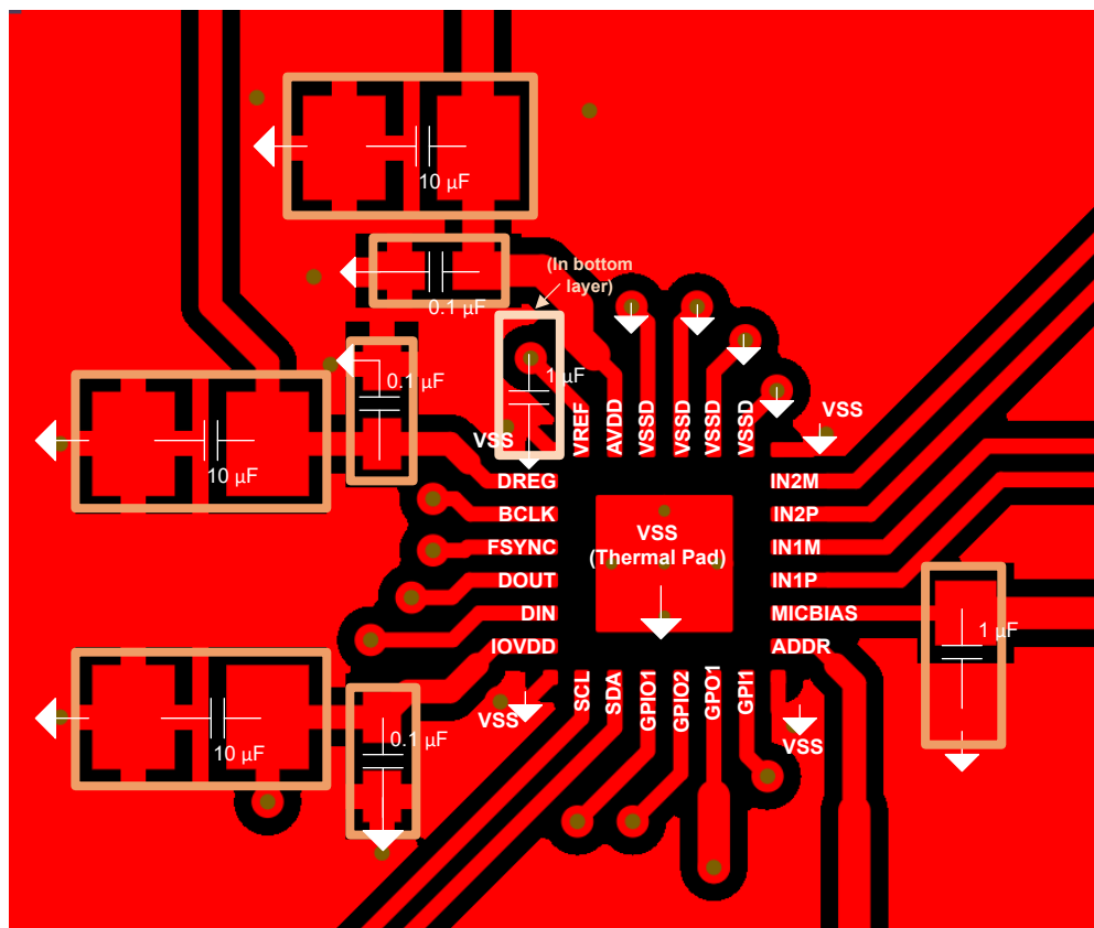
Figure 8-5. Example Layout
