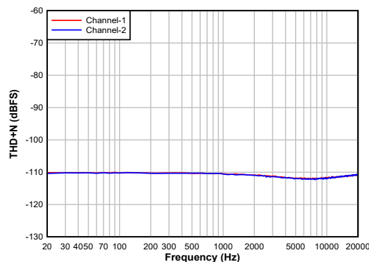
AC-coupled single-ended line input ( -60\text{dBFS} )
