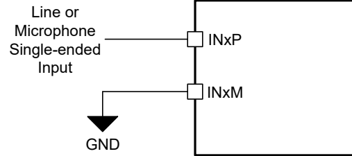
Figure 6-18. Single-ended DC-Coupled Input Connection (ADC_CHx_INSRC set to 2'b01 and ADC_CHx_CM_TOL set to 2'b01 or 2'10)
