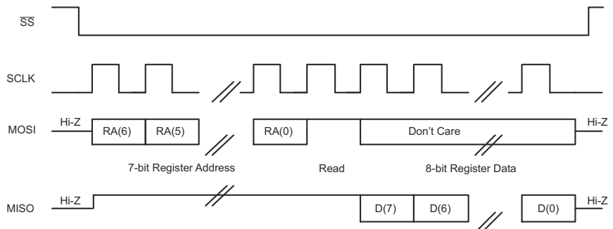
Figure 6-72. SPI Single-Byte Read Transfer
