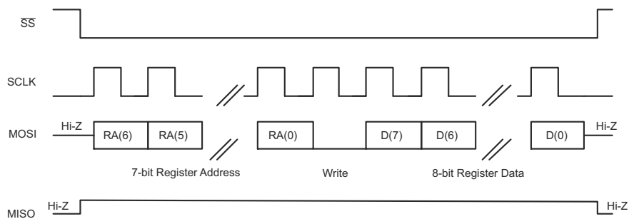
Figure 6-71. SPI Single-Byte Write Transfer
