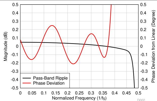
Figure 6-38. Low-Latency Decimation Filter Pass-Band Ripple and Phase Deviation
