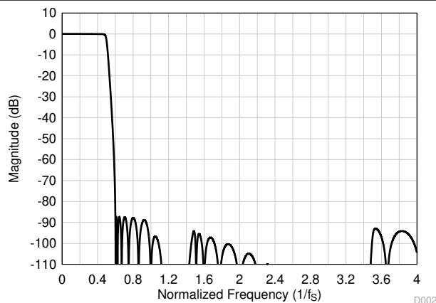
Figure 6-37. Low-Latency Decimation Filter Magnitude Response
