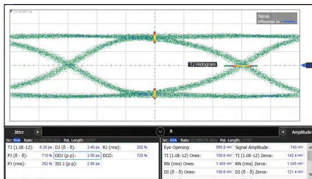
Figure 5-4. 32 Gbps 800 mV PRBS15 Source (1dB Loss)
