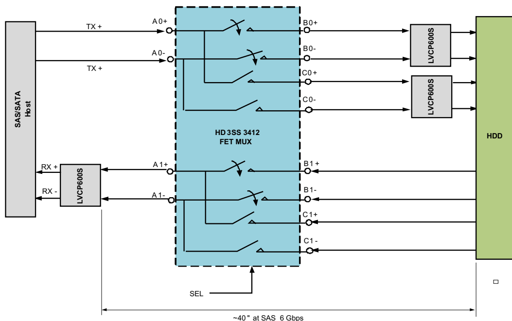
Figure 13. Typical Application
