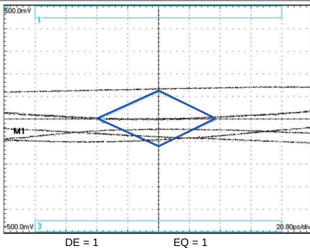
Figure 21. Eye Pattern at A → X = 40"; Y = 2"
