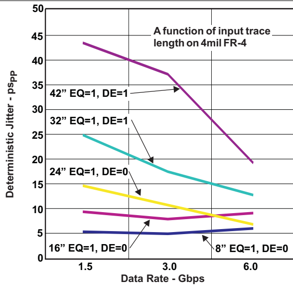
Figure 4. Deterministic Jitter vs Data Rate
