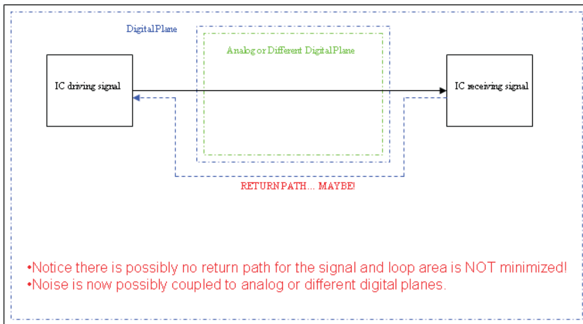
Figure 24. Incorrect Routing
