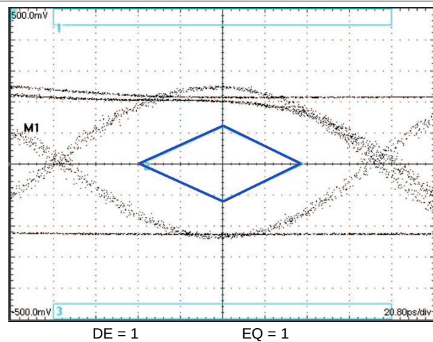
Figure 22. Eye Pattern at B → X = 40"; Y = 2"
