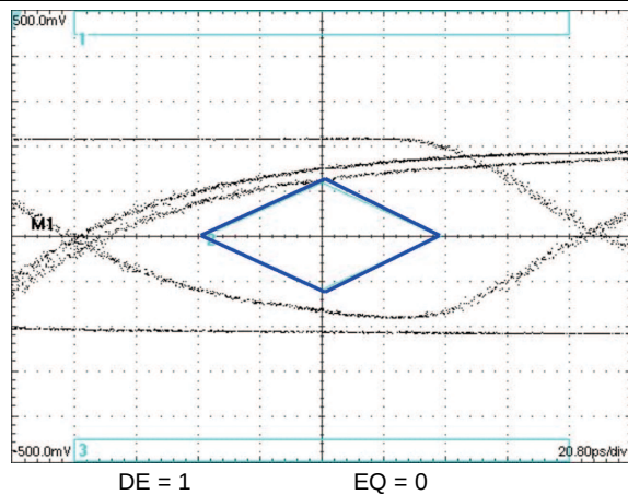
Figure 13. Eye Pattern at A → X = 8"; Y = 2"
