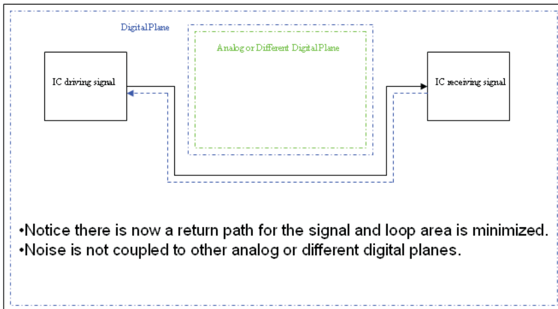
Figure 25. Proper Routing
