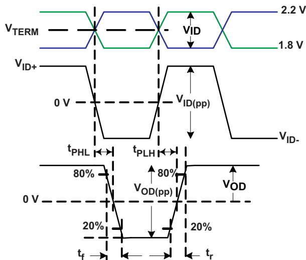
Figure 11. TMDS Main Link Timing Measurements
