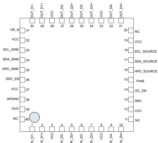
40-Pin WQFN RSB Package (Top View)
