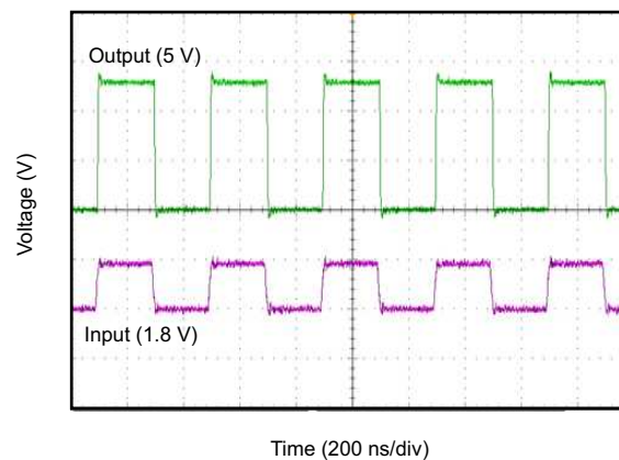
Figure 4. Translation Up (1.8 V to 5 V) at 2.5 MHz
