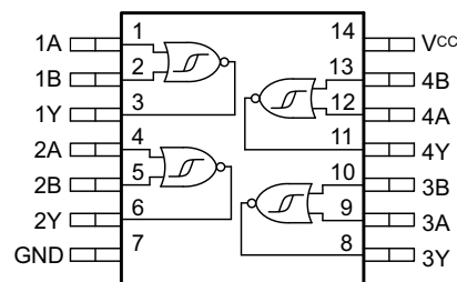
Logic Diagram
