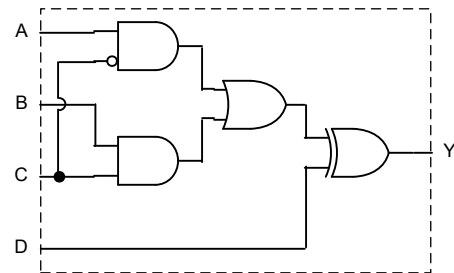
Figure 7-2. Configurable logic
