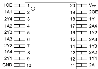
Figure 4-2. SN74LVC241A PW, DGS Package (Top View)
