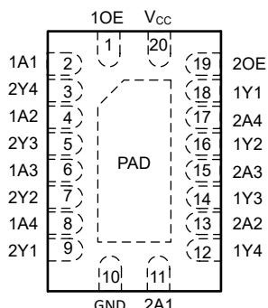
Figure 4-1. SN74LVC241A RKS Package (Top View)
