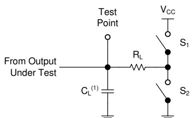
Figure 6-1. Load Circuit for 3-State Outputs
