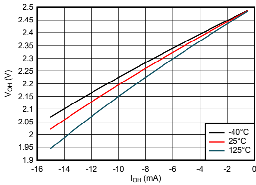
Figure 5-20. Output Voltage vs Current in HIGH State; 2.5V Supply
