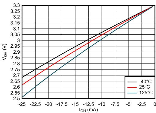
Figure 5-18. Output Voltage vs Current in HIGH State; 3.3V Supply
