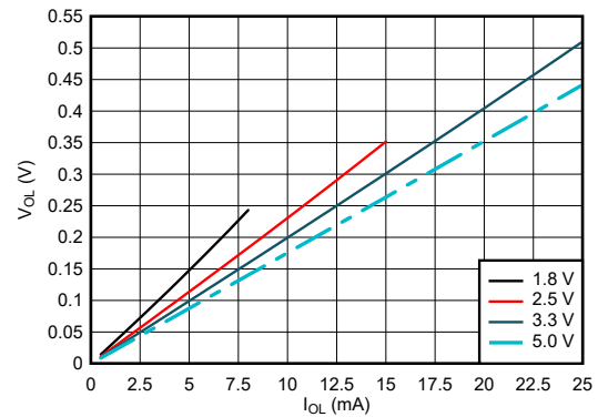
Figure 5-15. Output Voltage vs Current in LOW State
