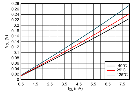
Figure 5-23. Output Voltage vs Current in LOW State; 1.8V Supply
