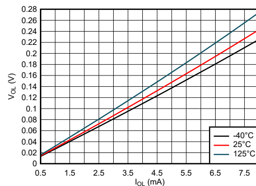
Figure 5-10. Output Voltage vs Current in LOW State; 1.8V Supply
