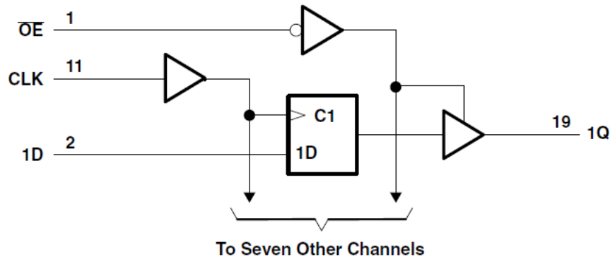
Logic Diagram (Positive Logic)
