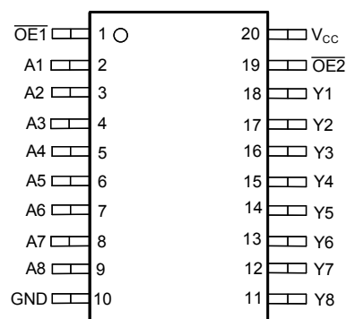
Figure 5-2. DGS Package, 20-Pin SOT (Top View)
