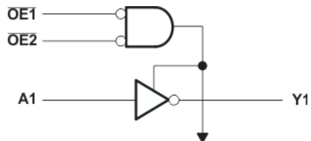
Figure 3-1. Simplified Schematic
