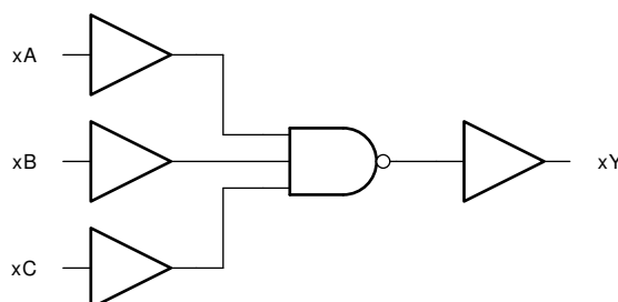
Figure 8-1. Simplified Schematic
