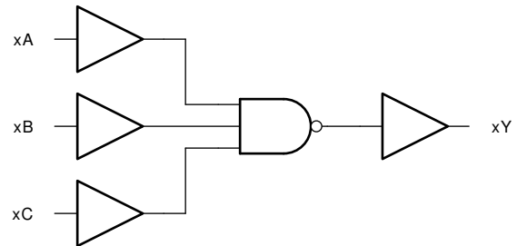
Simplified Schematic
