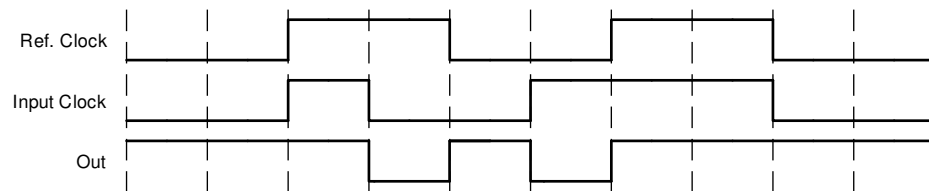
Figure 10. Application timing diagram
