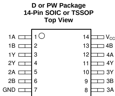
Pin Functions
