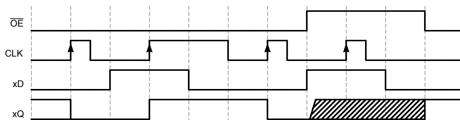
Figure 6-1. Timing diagram
