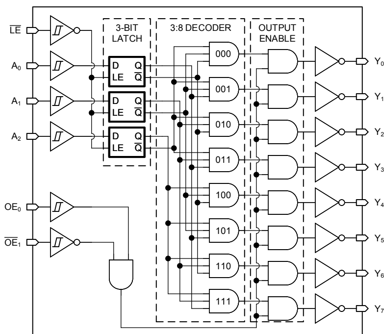
Figure 8-1. Logic Diagram (Positive Logic) for the SN74HCS137
